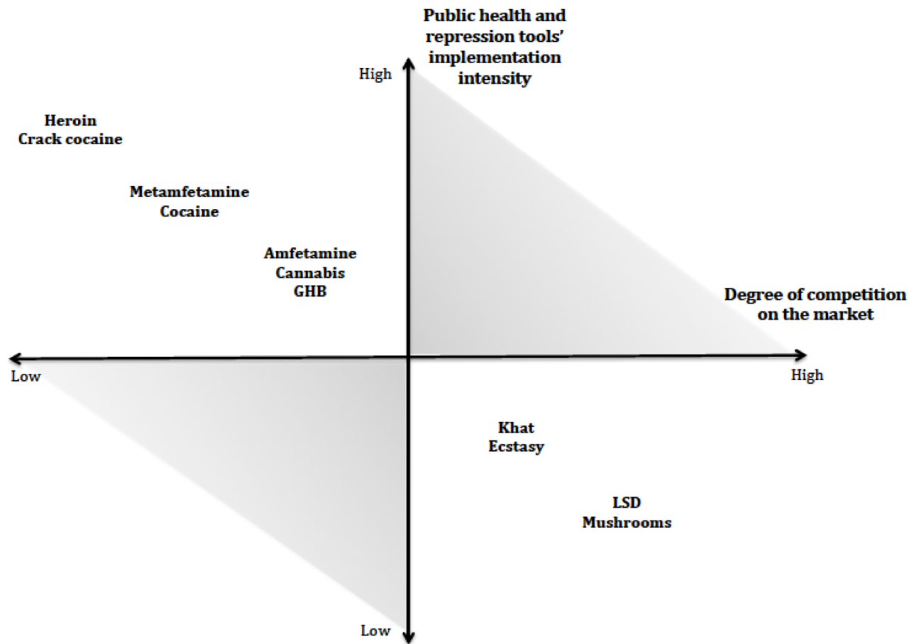
Figure 1. Public health and repression tools' implementation intensity and degree of competition on the market based on the substances' estimated potential for harm, by Nutt et al. (2010).
